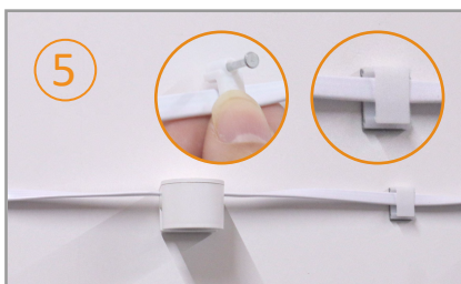
5 Secure the power cord with snap or staple clips
